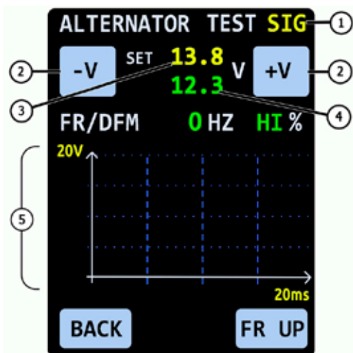
Fig. 8. Diagnostic screen for alternators of type "COM" of 24V.
