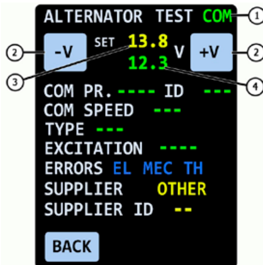
Fig. 7. Diagnostic window of the "COM" of 12V type alternator.
